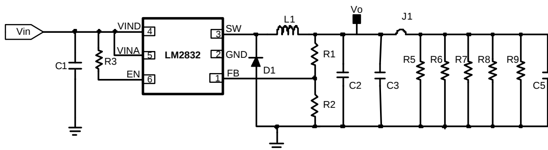
Figure 1. LM2832X 6-Pin WSON Demo Board Schematic
